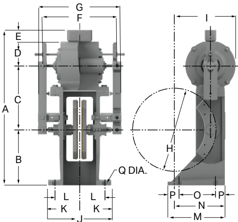
DIMENTIONS (INCHES)
