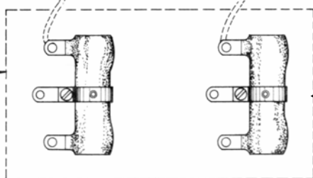
LC27-0002N RESISTOR KIT,440-550 V for "RPR-1" reverse phase relay (2) 10K OHM 25W
