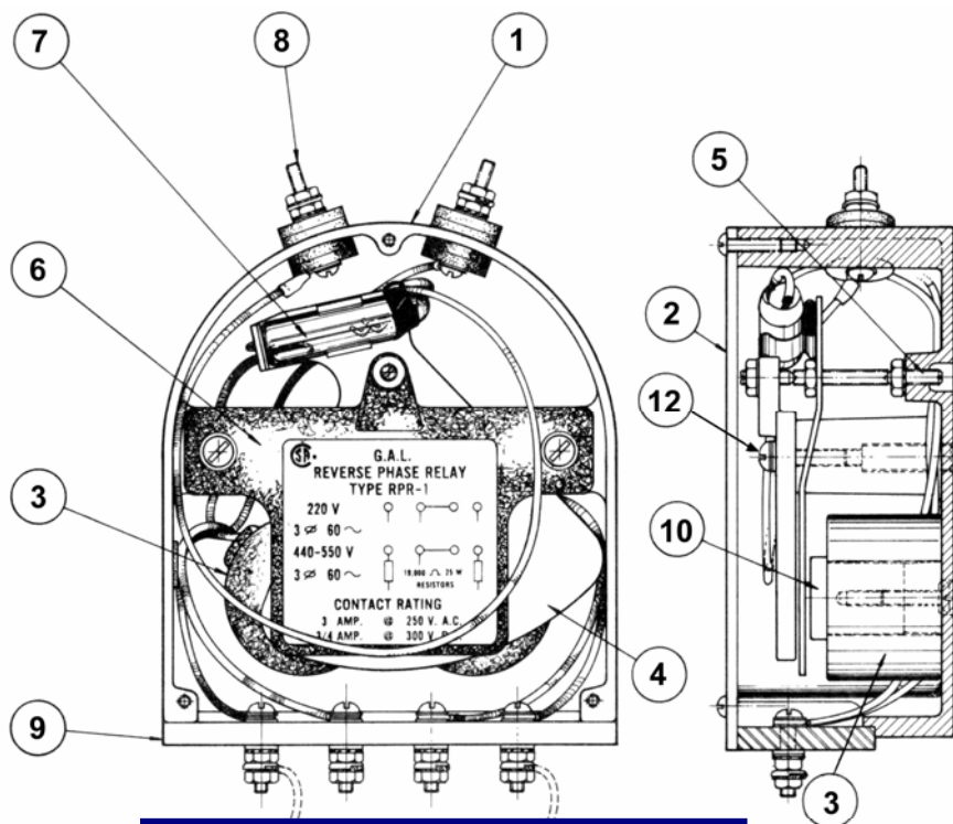
LC27-0001N RELAY,"RPR-1" REVERSE PHASE
